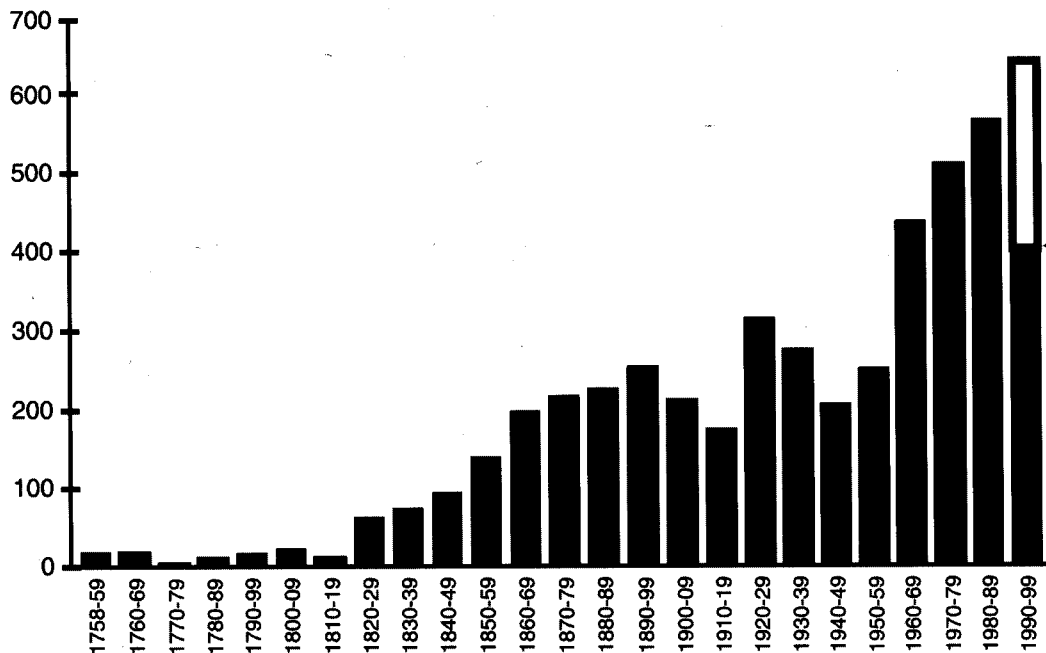
Figure 2. Amphibian species descriptions since 1758 (synonyms not included), clustered by decade, from Claw and Köhler (1998). The arrow indicates the end of 1995; descriptions for the period 1996–1999 were extrapolated.
