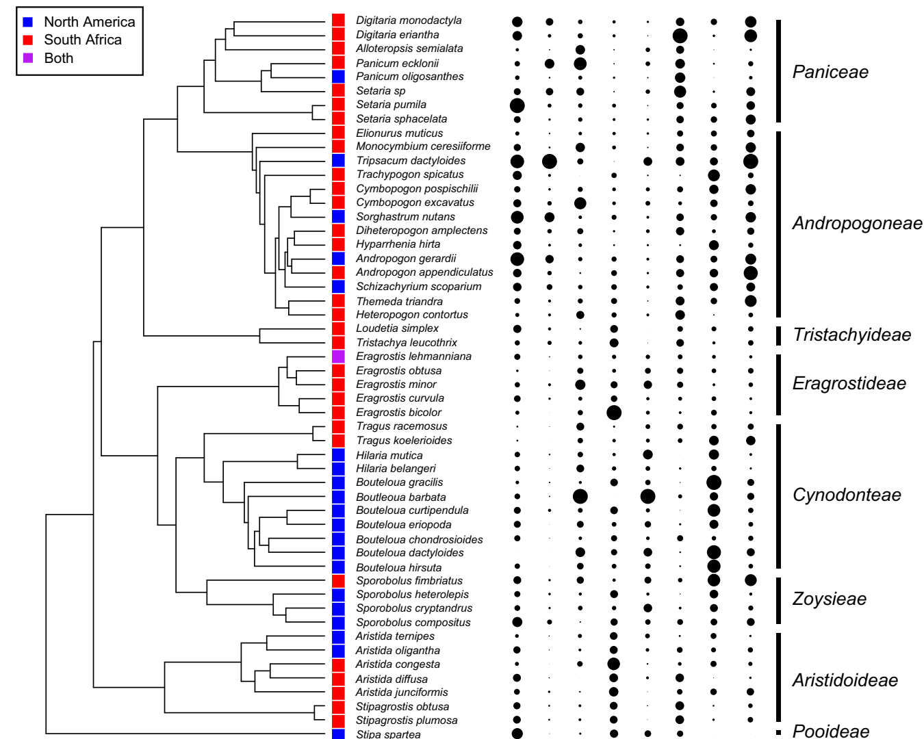
Fig. S4. Phylogeny of dominant species in NA and SA sites with a subset of trait values mapped onto the tips. Trait values are scaled between zero and one, and larger circles indicate larger values.
