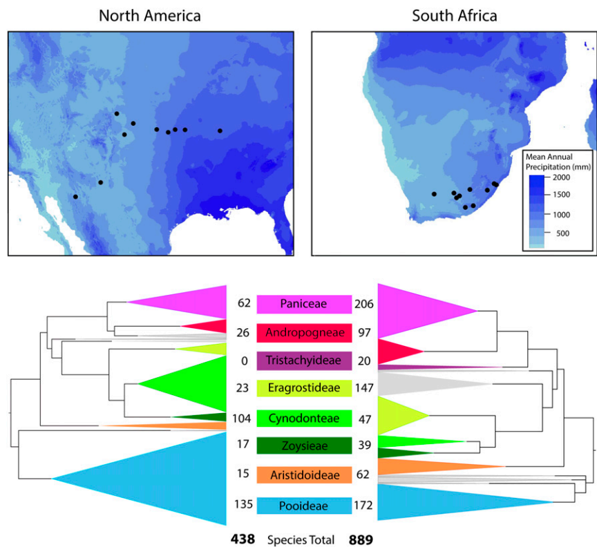
Fig. S1. Regional Poaceae clade richness, using GPWG (39) as a backbone tree and grafting on the species for each clade, size of clades represent proportion of total richness of that clade.
